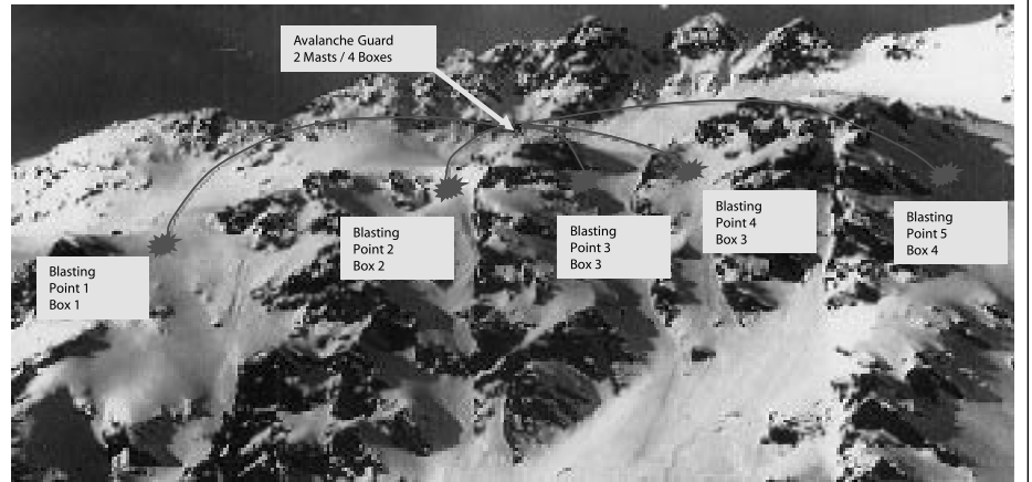
Typical Avalanche Guard Setup
