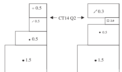
Figure 3. Two profiles with similar strength and energy, but different structural properties.
