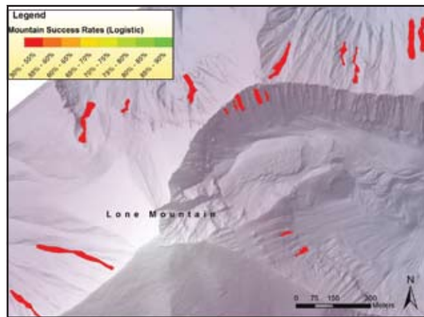
Figure 2: Success rates for a model of all depth hoar PTLs on Lone Mountain. The model does little better than a coin toss, suggesting that we can't apply a rule of thumb for locating PTLs using terrain.
