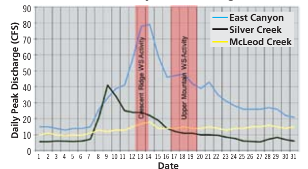
March 2007: Daily Peak Discharge Levels
