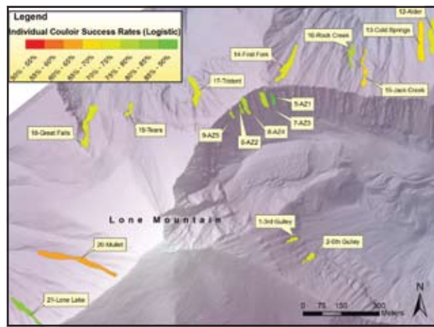
Figure 1: Success rates for models of depth hoar PTLs for each individual couloir on Lone Mountain, MT. The relatively high success rates indicate that terrain has a strong relationship with PTLs.
