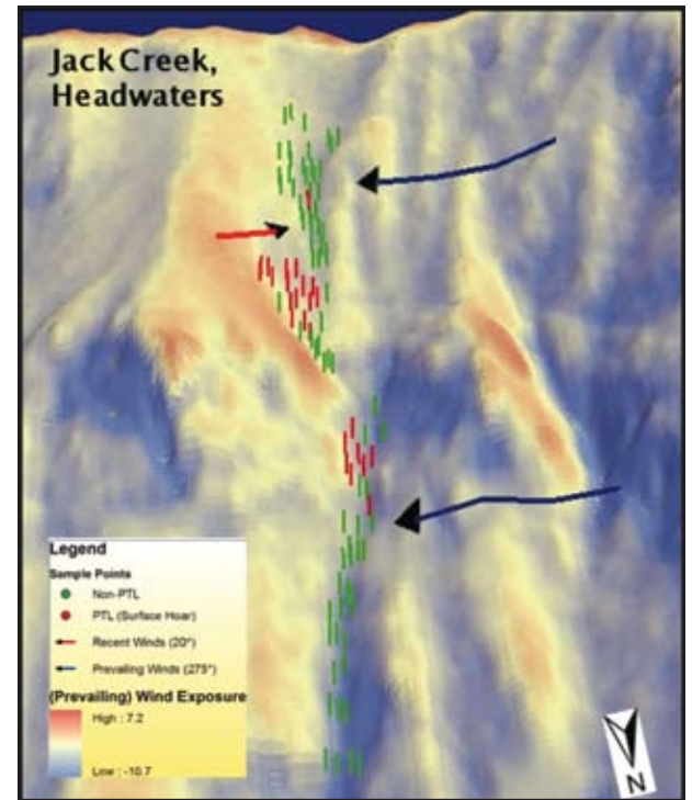
Figure 6: Distribution of surface hoar PTLs in Jack Creek Couloir. Surface hoar was preserved in areas that are normally exposed to prevailing winds. This illustrates how an understanding of previous weather and wind patterns is needed to use terrain to predict PTLs.
