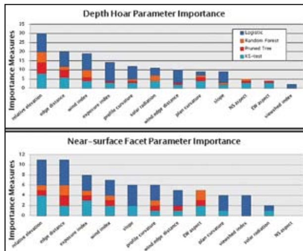
Figure 3: Relative importance measures for each of the twelve terrain parameters used to model PTLs. The different colors represent different model structures. The top four parameters for both depth hoar PTLs and near-surface facet PTLs are all related to wind loading and scouring patterns.
