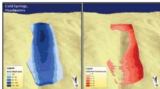
Figure 4: Distribution of snow depth and depth hoar on one of the slopes. This illustrates how a physical process, such as temperature gradients causing faceting, can be used in relation with terrain to predict weak layer presence.
